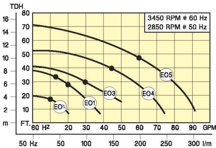
PUMPE 'EO'
